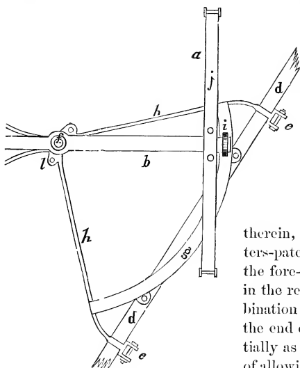
EVERETT'S PERCH-COUPLING.
